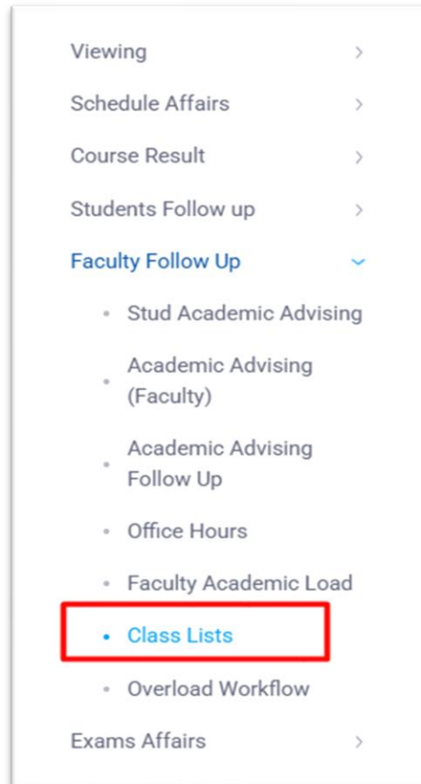
Figure 1- Class List
