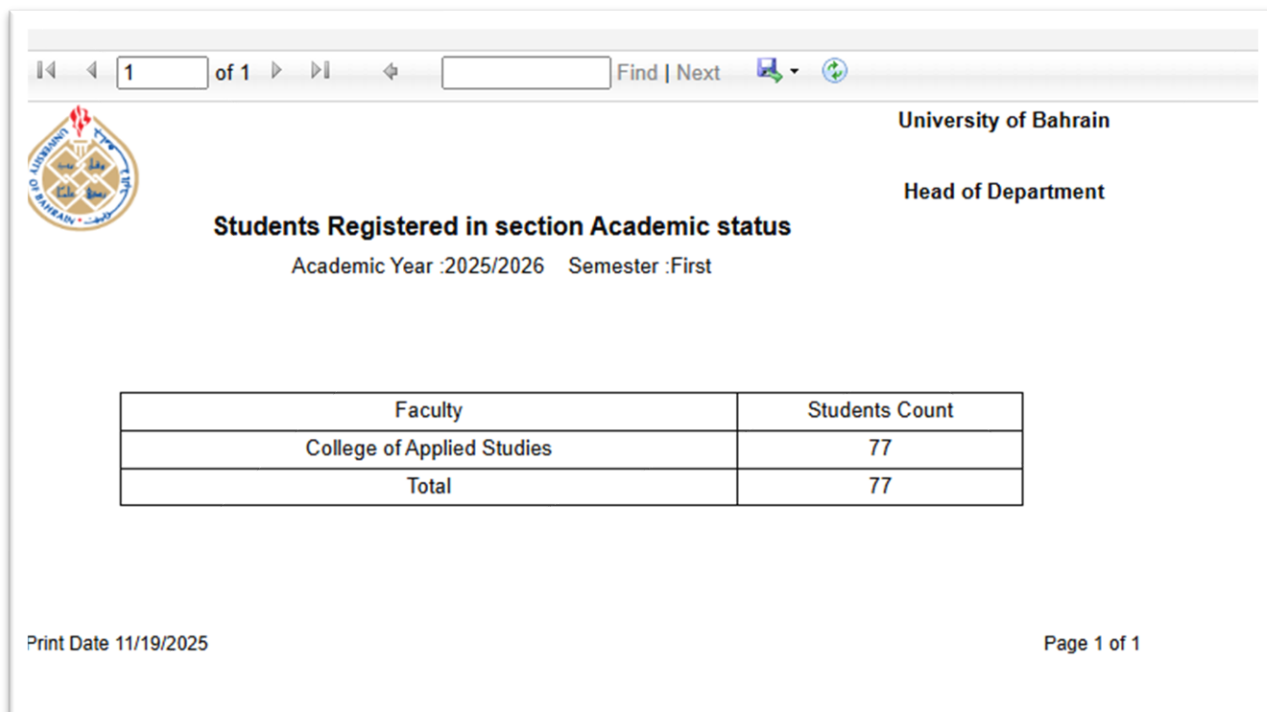
Figure 4- Statistical Report
