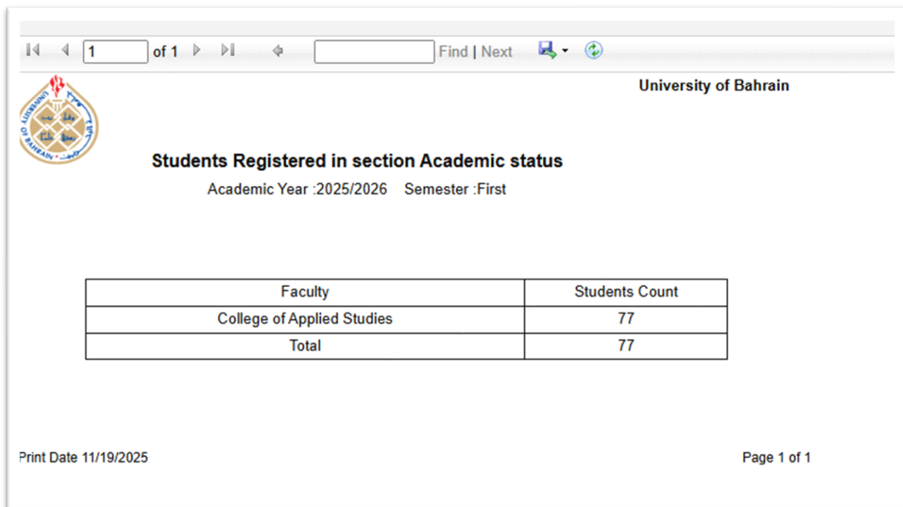
Figure 4- Statistical Report
