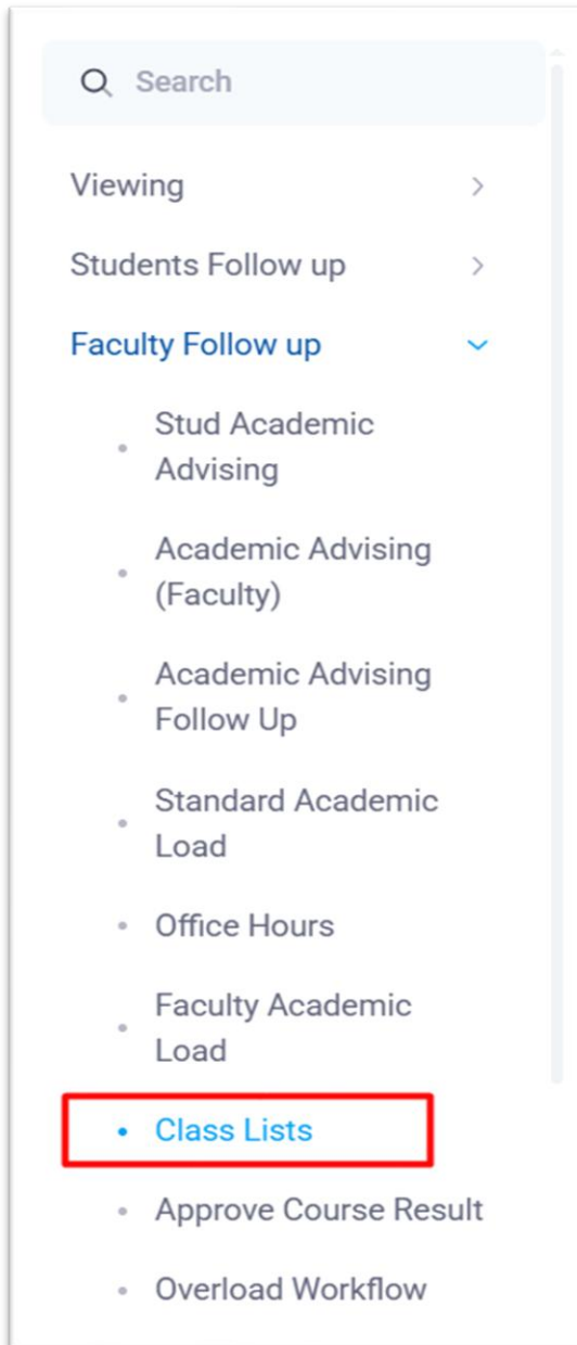
Figure 1- Class List
